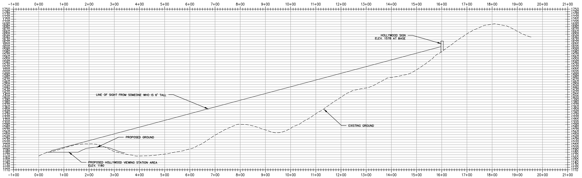
HOLLYWOOD SIGN VIEWING STATION TO HOLLYWOOD SIGN PROFILE
